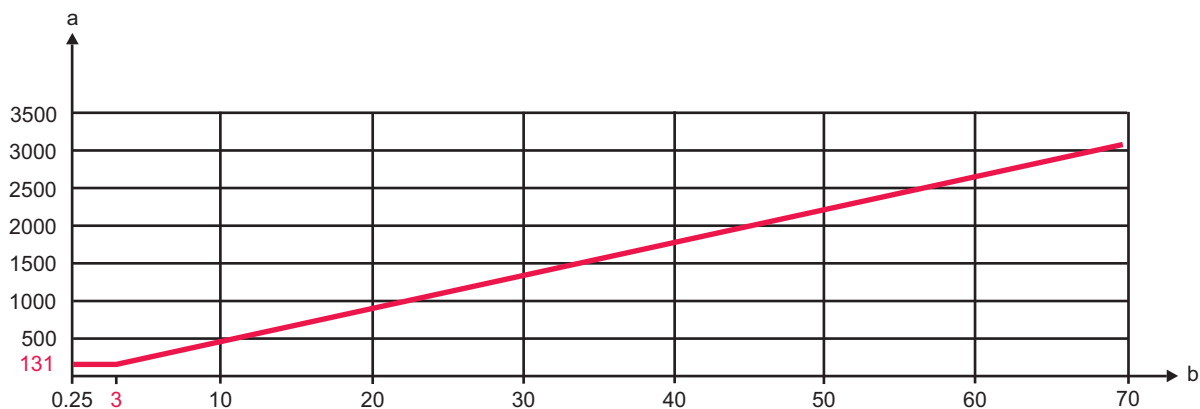
Fig. 4.3: Minimum distance to reflective surfaces as a function of the protective field width up to 10 m
